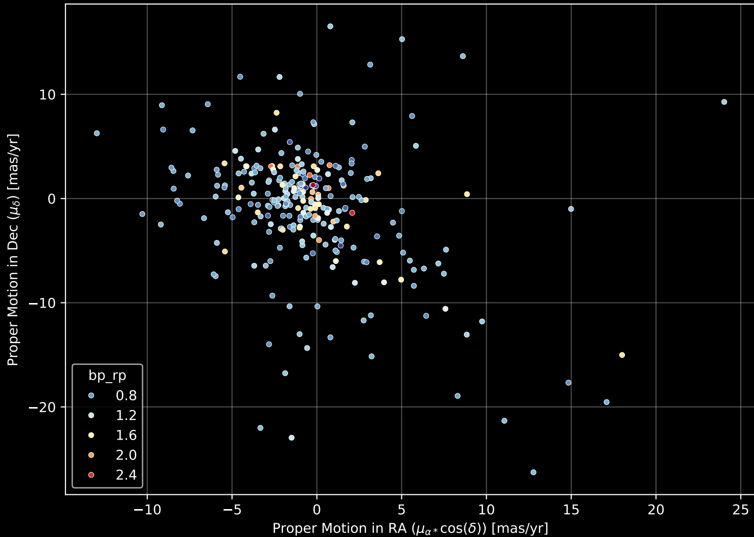
GALAH DR4 Field: [8893] Proper Motion Diagram (n= 272)
