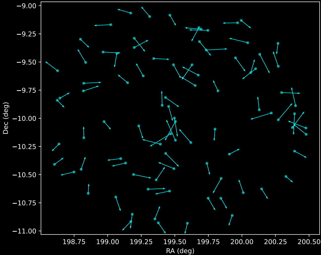
GALAH DR4 Noise Stream Proper Motion Vectors (n=88)
