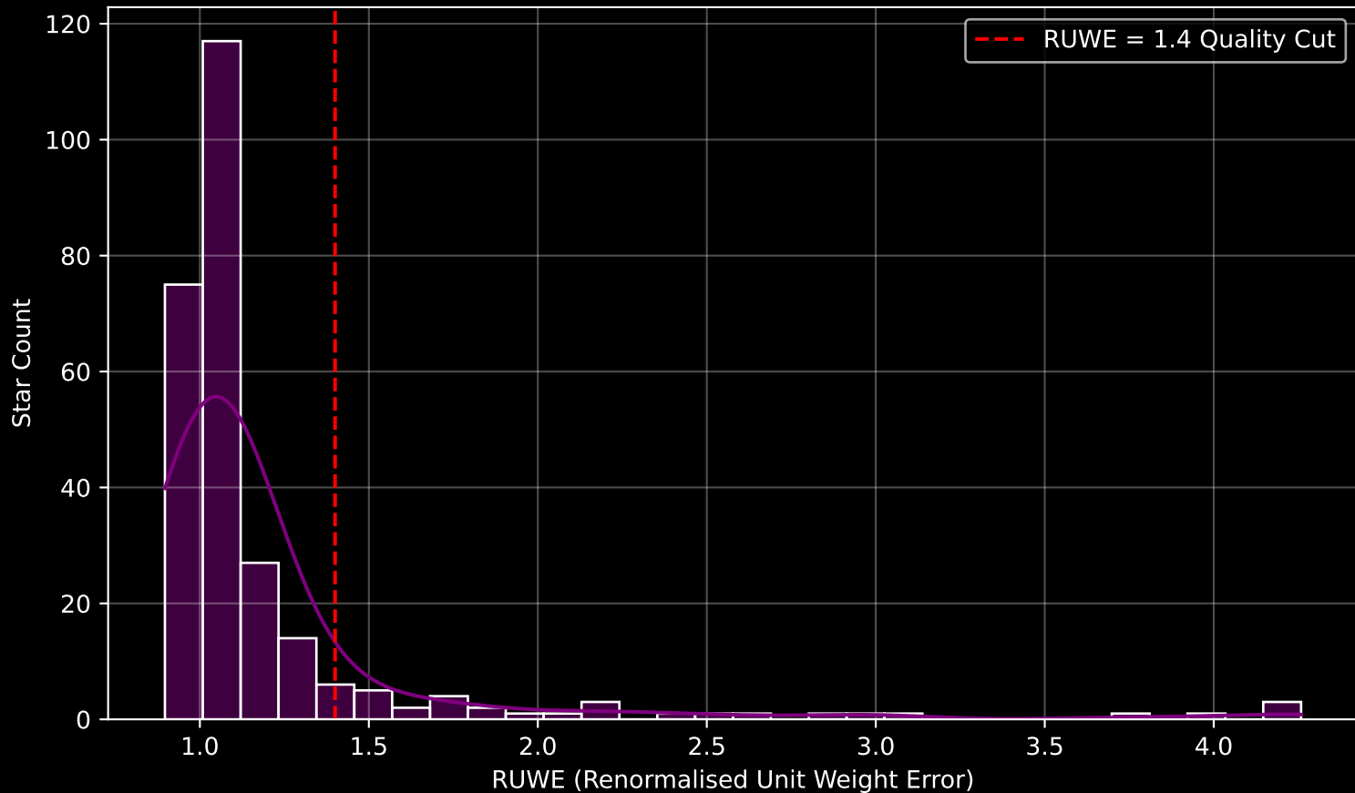
GALAH DR4 Field [8893] RUWE Distribution (n= 268)
