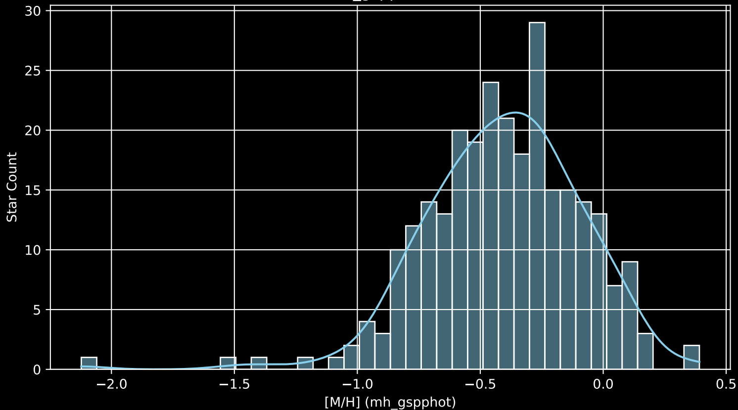
GALAH DR4 Field: [8893] [M/H] (mh_gspphot) (n= 272)
