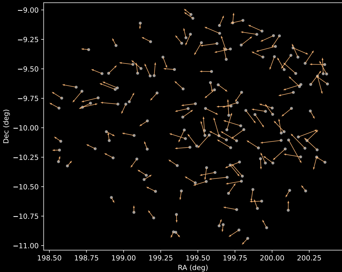
GALAH DR4 Cluster 3 Proper Motion Vectors (n=158)
