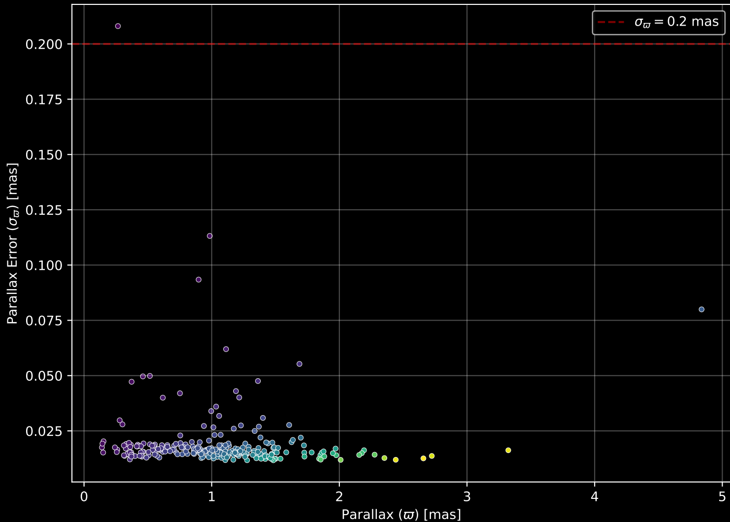
GALAH DR4 Field: [8893] Parallax Quality (n= 272)
