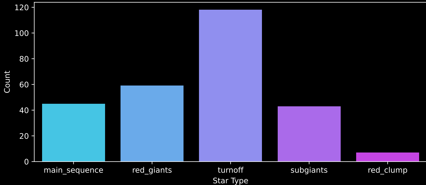
GALAH DR4 Field: [8893] Count plot of Star Type
